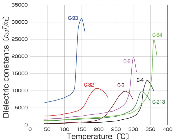
Dielectric constants Vs Temperature
